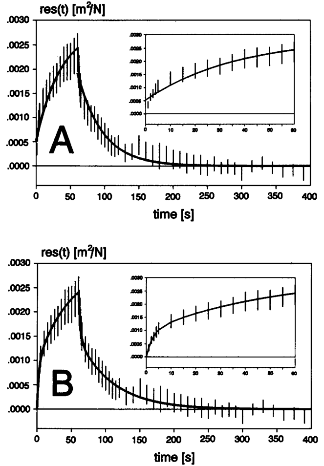
FIGURE 3 Fitting of the function (Eq. 17) (A) and of the biexponential function (Eq. 18) (B) to the experimental data for the whole experimental period and for the first 60 s (inserts) of the experiment. Vertical bars are standard deviations of determined creep values. They determine the width of the area, equal [s^2]^{1/2}(t) where all the expected trajectories of creep for most cells in the population will be found. The function corresponding to the proposed biexponential rheological model passes through this area (solid line), as proved by the \chi^2 test.
