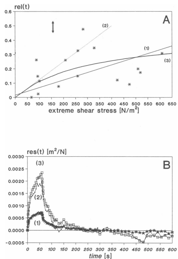
FIGURE 2 Illustration of fitting procedures for determining the response function. (A) Fitting procedures in the 15th s of the experiment. Experimental values of the relationship of rel(t) to \sigma_t^{ext} for all cells at a given time point were analyzed by various fitting procedures: (1) linear regression for all data (see text, procedure a) (2) linear regression, for data obtained under small stress (see text, procedure b) (3) nonlinear regression according to Eq. 14. rel(t) values greatly vary for different cells under similar stress. The bidirectional arrow represents the mean error of experimental measurements of deformations. (B) Response functions obtained from the experimental data analyzed according to Fig. 2A for all time points, following the three proposed regression procedures. The respective values of res(t) are denoted by geometrical symbols.
